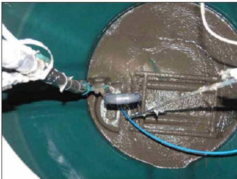
Figure 2.2 Floating scum layer inside the reactor vessel of a 'Balmoral' septic tank as viewed from above. The tubing forms part of the "air lift" pump system that transfers effluent between the chambers and pumps clarified effluent out of the system (Image courtesy of J Malley, National Trust).
