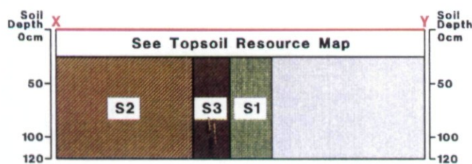
Diagrammatic Section across Site
