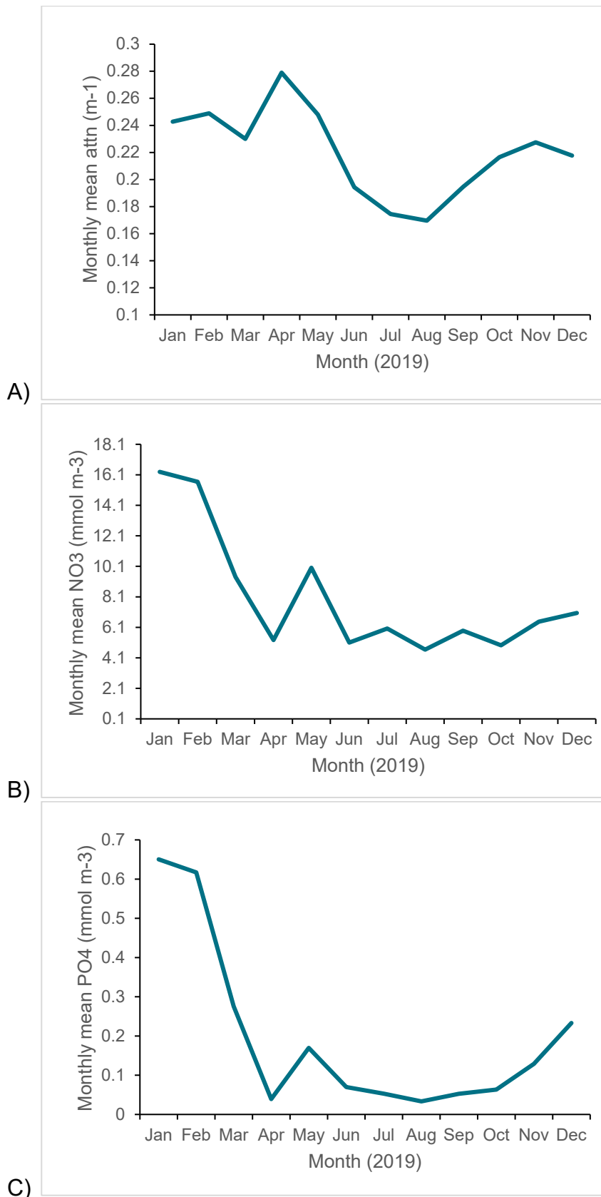
Figure 5: The monthly averages for modelled light attenuation co-efficient (attn (a)) and nutrient (nitrate NO 3 (b) and phosphate PO 4 (c)) data for the Essex Estuaries SAC. Data source code 4, see section Dataset sources . Graphs generated using E.U. Copernicus Marine Service Information.
