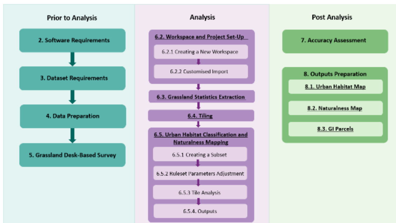
Figure 5. Diagram showing the steps in the Urban Habitat and Naturalness Mapping approach.
