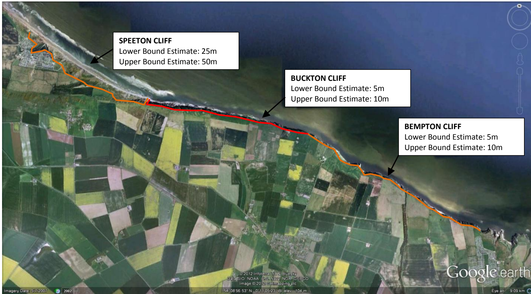
Figure 5 Flamborough Head SSSI (Reighton to Long Ness): predicted 50-year recession rates of site boundaries (Image source: Google Earth). The coloured lines show the approximate cliff unit boundaries.
