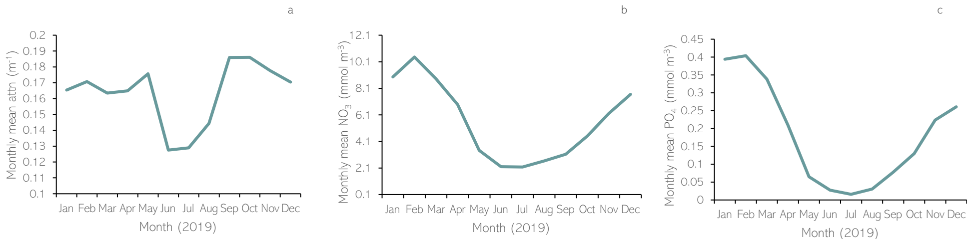
Figure 3 - The monthly averages for modelled light attenuation co-efficient (attn (a)) and nutrient (nitrate NO_3 (b) and phosphate PO_4 (c)) data for the Plymouth Sound and Estuaries SAC (4)
