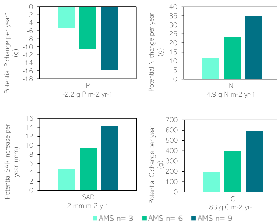
Figure 4 - Potential change in ecosystem services based on replacing 3, 6 and 9 swing moorings with advanced mooring systems (AMS). N=Nitrogen, P=Phosphorous, C=Carbon, SAR=Sediment Accumulation Rate.
