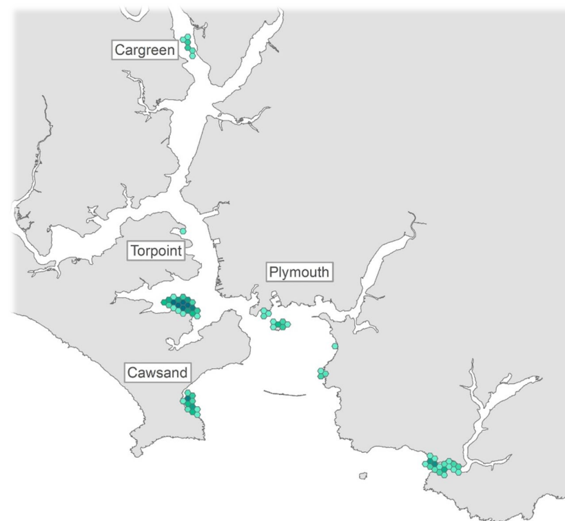
17. The current distribution of seagrass within the Plymouth Sound and Estuaries SAC
