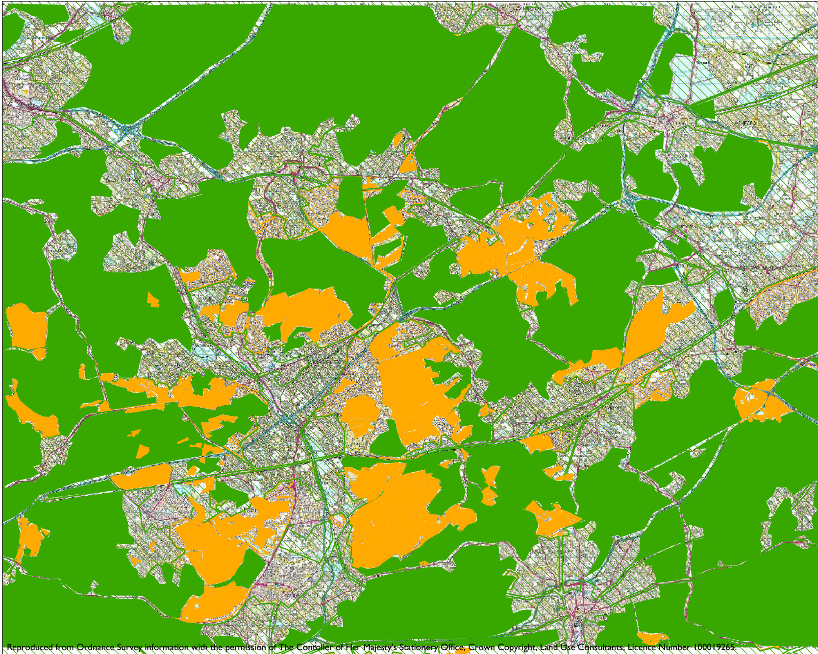
Map 4.5: Loss of Heathland and Open Land between 1904-2003
